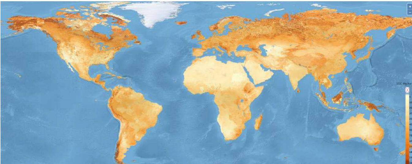
Figure 3 – Global soil organic carbon map (Source: FAO & ITPS 2018)
